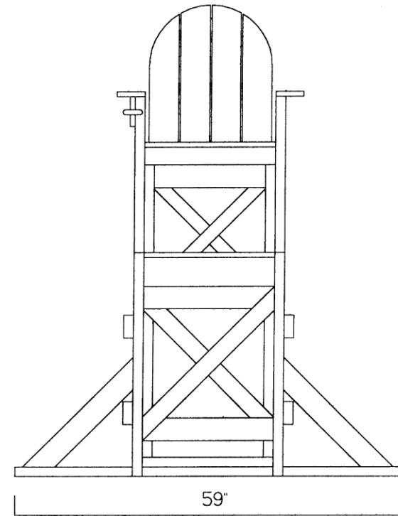
FRONT VIEW
