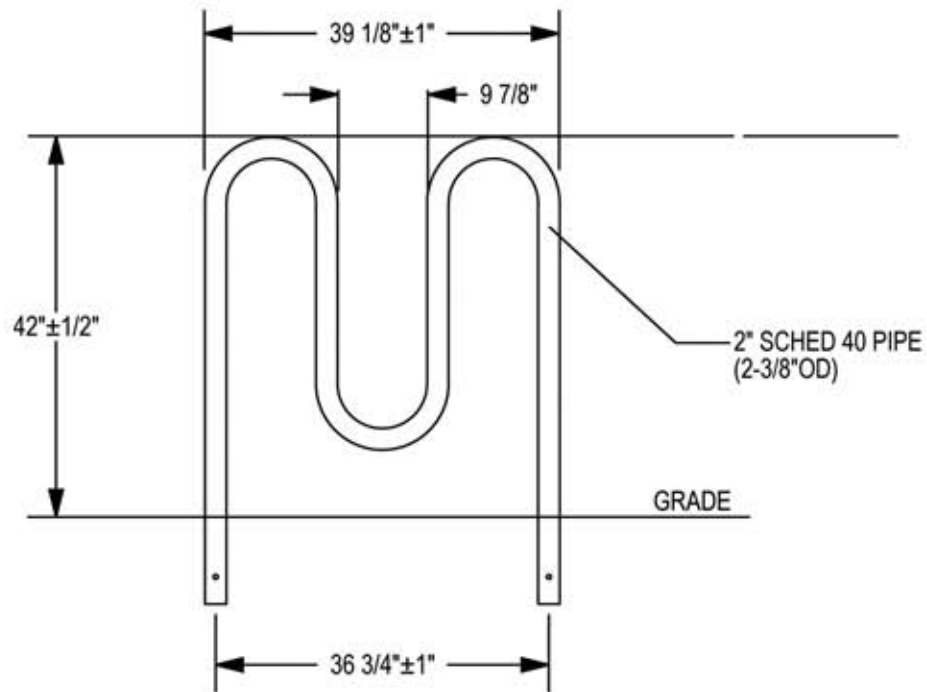
ELEVATION VIEW
