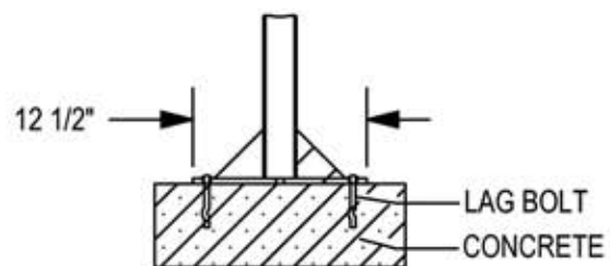
□ SURFACE GUSSET MOUNT (SG)
