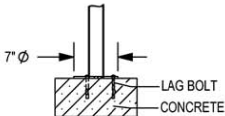
□ SURFACE FLANGE MOUNT (SF)
