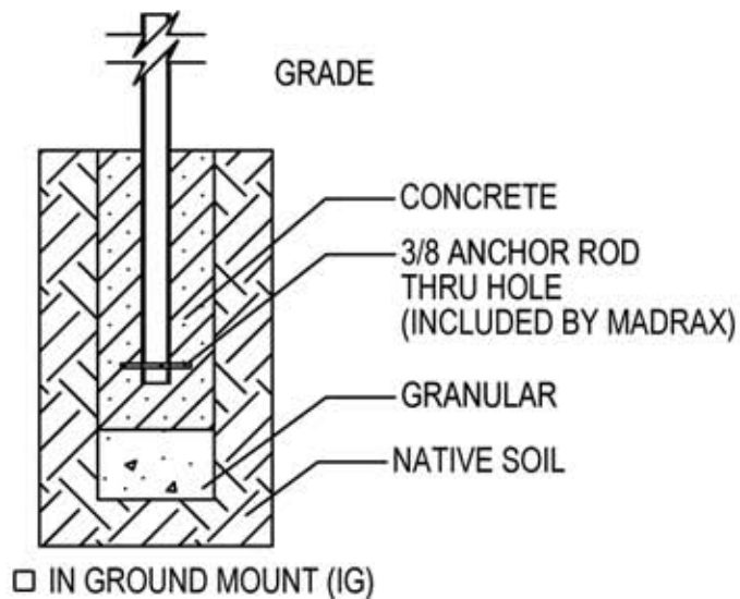
ELEVATION VIEW
